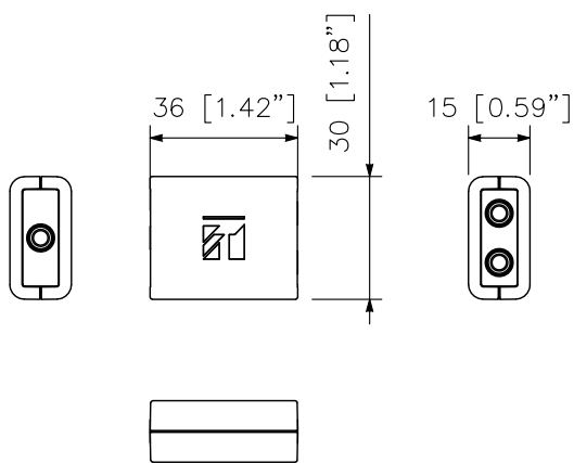
Distributor
